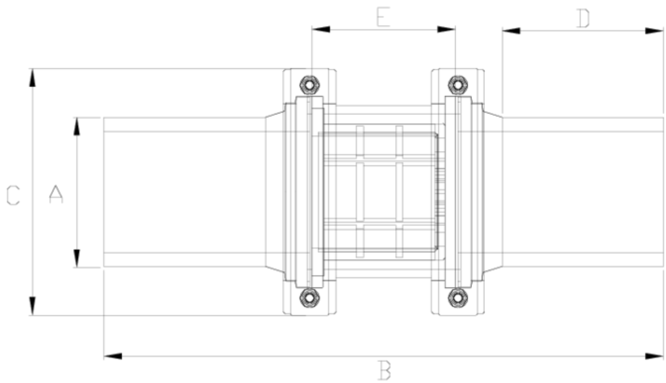
ITEM 517 | Line filter PE-PE outlet - screen sight glass
