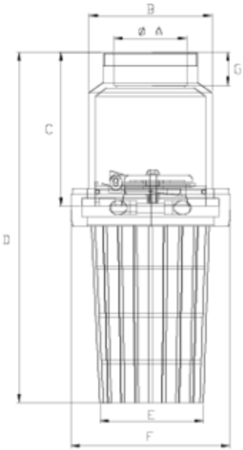
ITEM 294 | Flotation valve, Female/T
