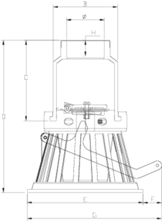
ITEM 290 | Foot valve, Female threaded outlet
